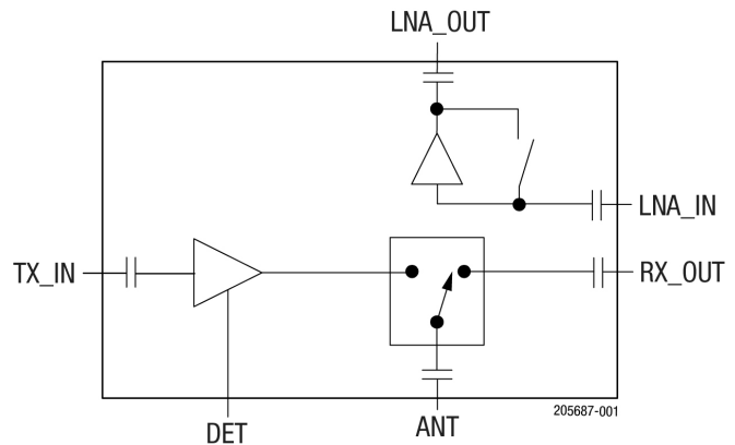
Figure 1. SKY85353-11 Block Diagram
