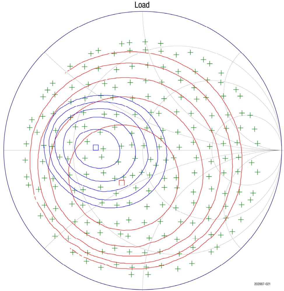
Figure 21. OIP3 Load Pull @ 1900 MHz, 5 V, 70 mA (Input Load = Min NF, -20 dBm/tone, 5 MHz Spacing)
